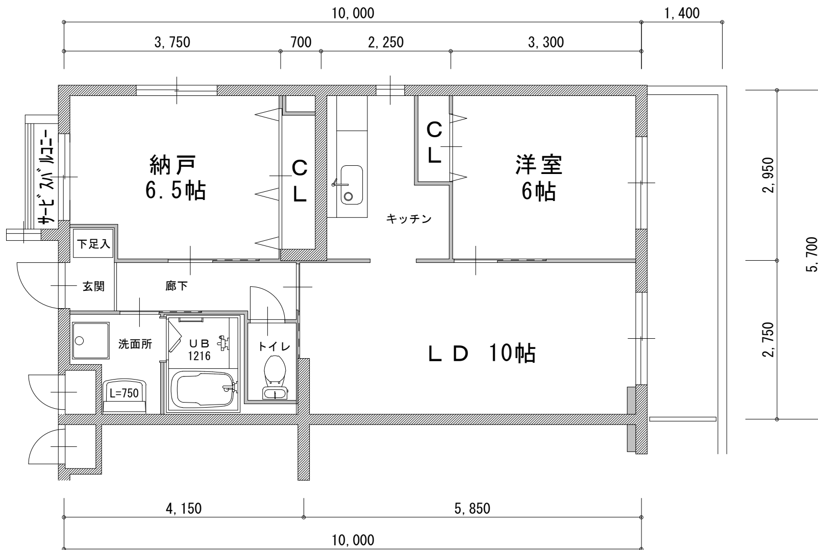
A 1 TYPE 56.46 m 2
