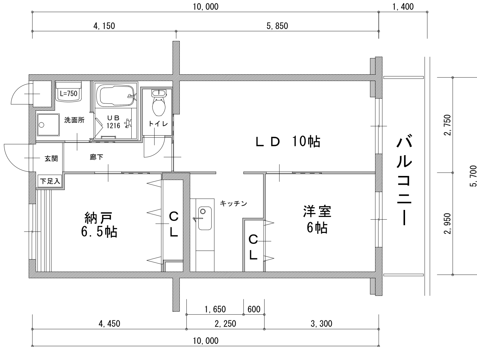
A 2 TYPE 55.33m 2
