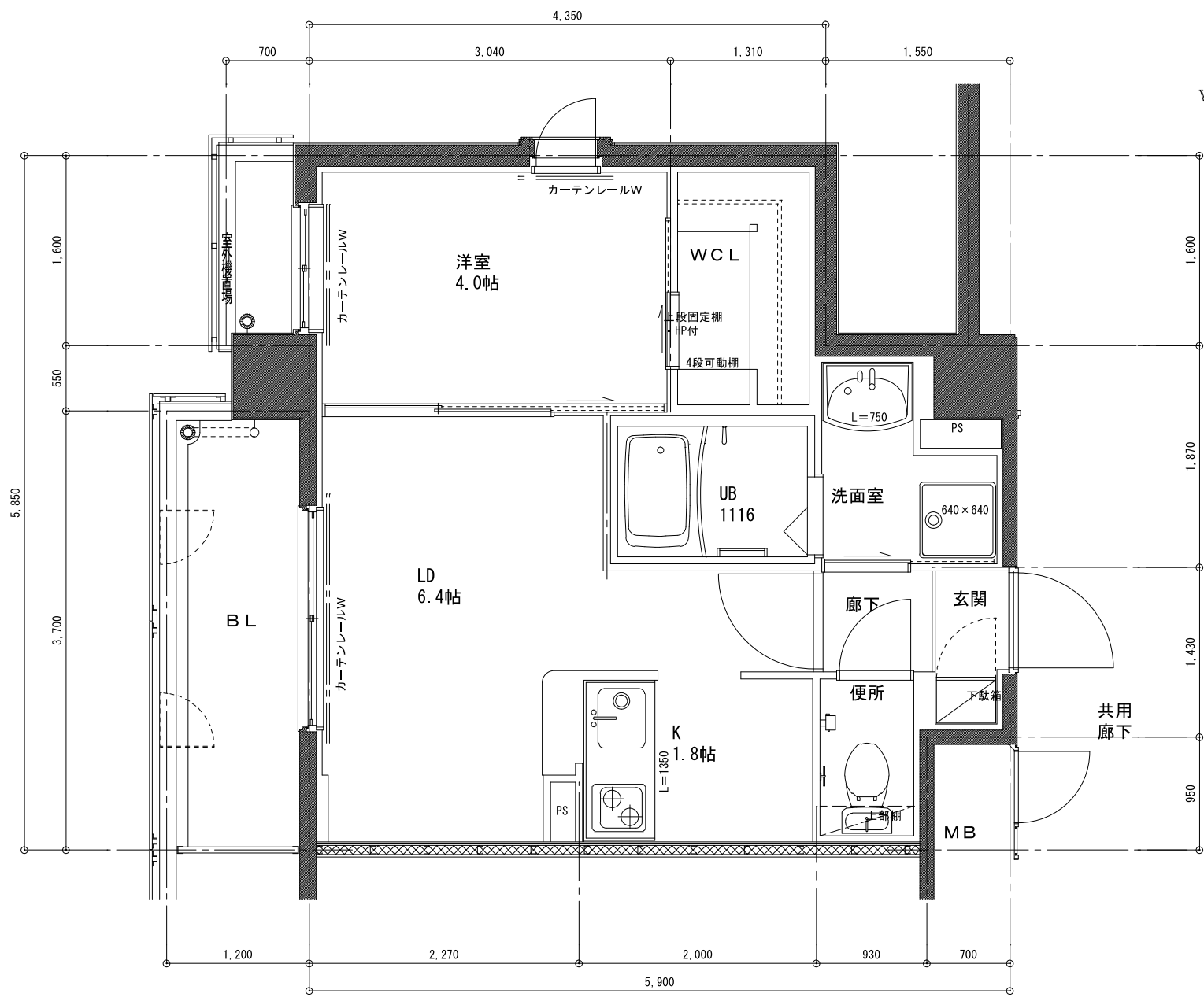
A TYPE 32.04㎡
